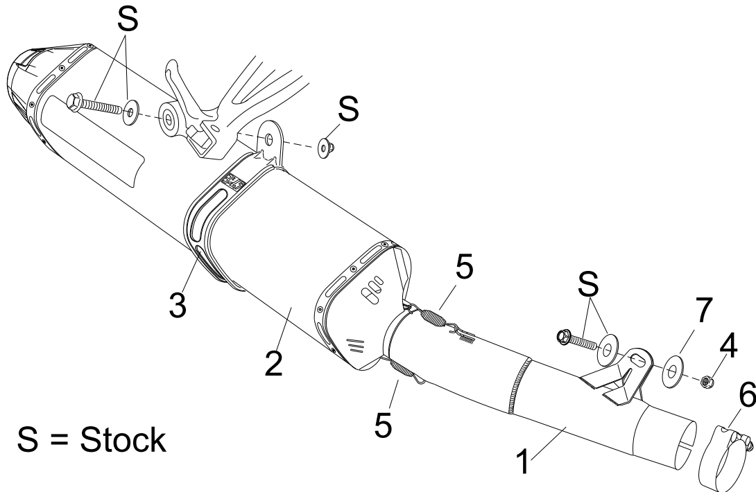
Parts Diagram
